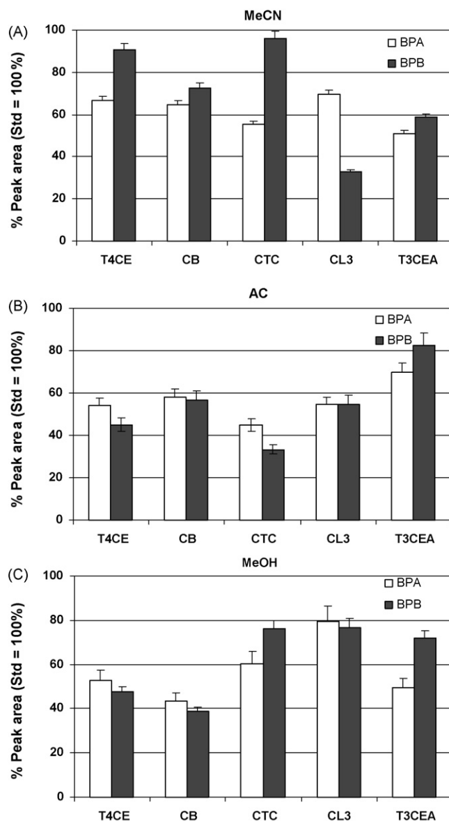
Fig. 4. Comparison of average peak area response of different dispersive solvents: (A) MeCN; (B) AC; and (C) MeOH, containing different extractive solvents (T4CE, T3CEA, CB, and CTC), normalized to the standard peak area (Std = 100%) ( n = 2 ).
