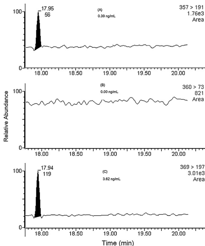
Fig. 1. MRM chromatograms of (A) free BPA, (B) d6-BPA, and (C) ^{13}\text{C}_{12} -labelled BPA of a serum sample not enzymatically deconjugated.
