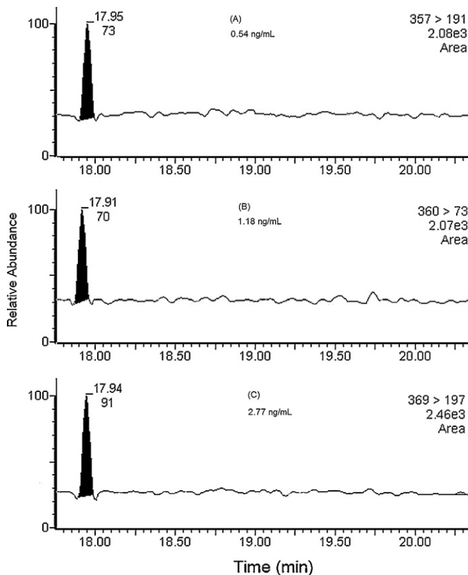
Fig. 2. MRM chromatograms of (A) free BPA, (B) d6-BPA, and (C) ^{13}\text{C}_{12} -labelled BPA of a serum sample enzymatically deconjugated with \beta -glucuronidase.
