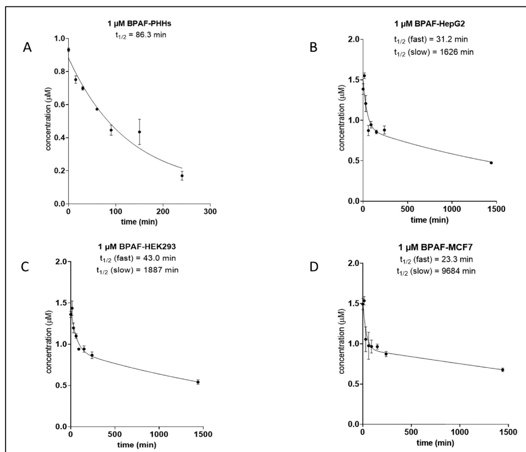
Fig. 4. Clearance of BPAF by PHH and three Tox21 cell lines.
