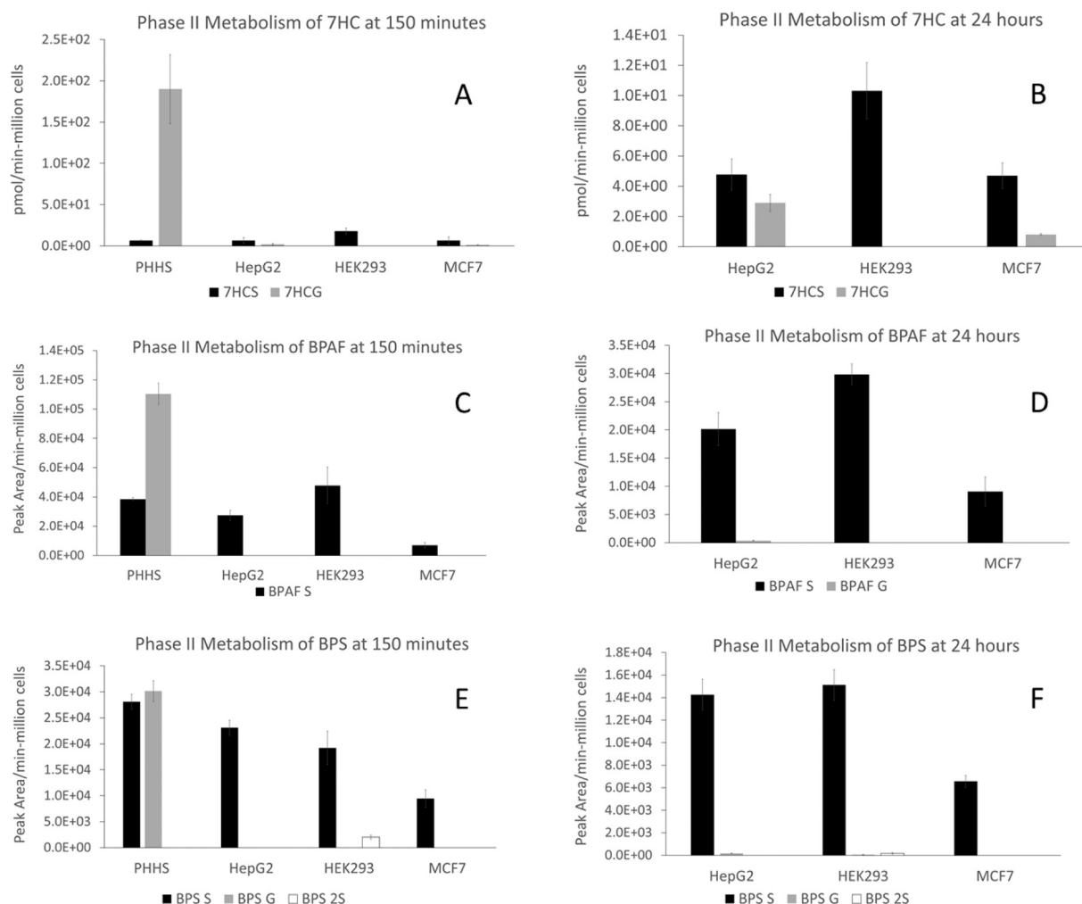
Fig. 2. Glucuronide and sulfate conjugates assay in PHH and three Tox21 cell lines.
