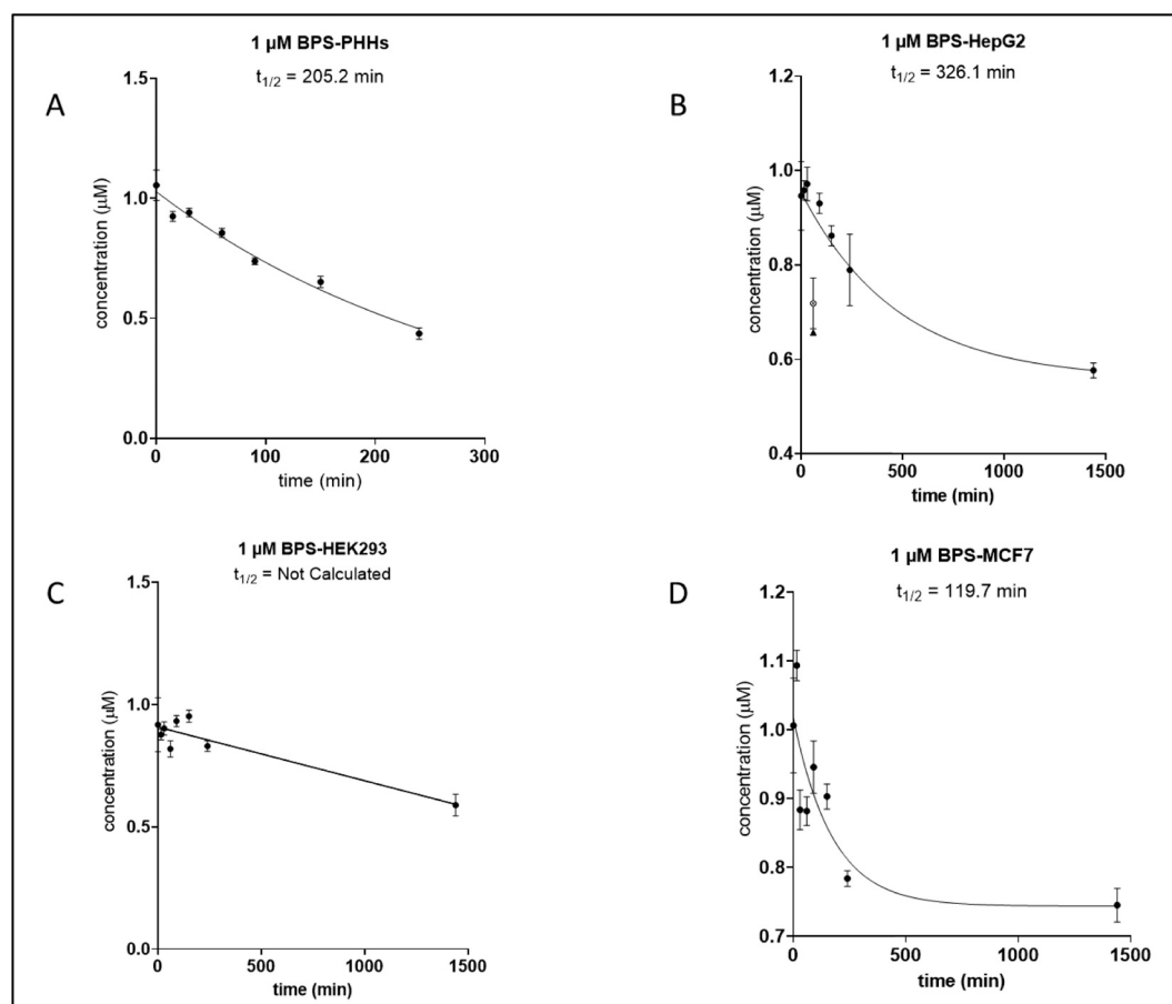
Fig. 5. Clearance of BPS by PHH and three Tox21 cell lines.
