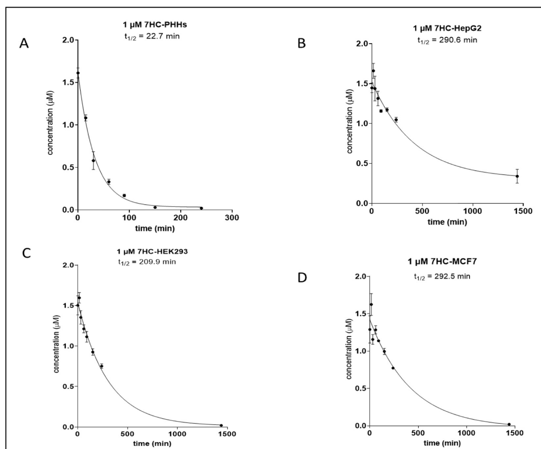
Fig. 3. Clearance of 7HC by PHH and three Tox21 cell lines.
