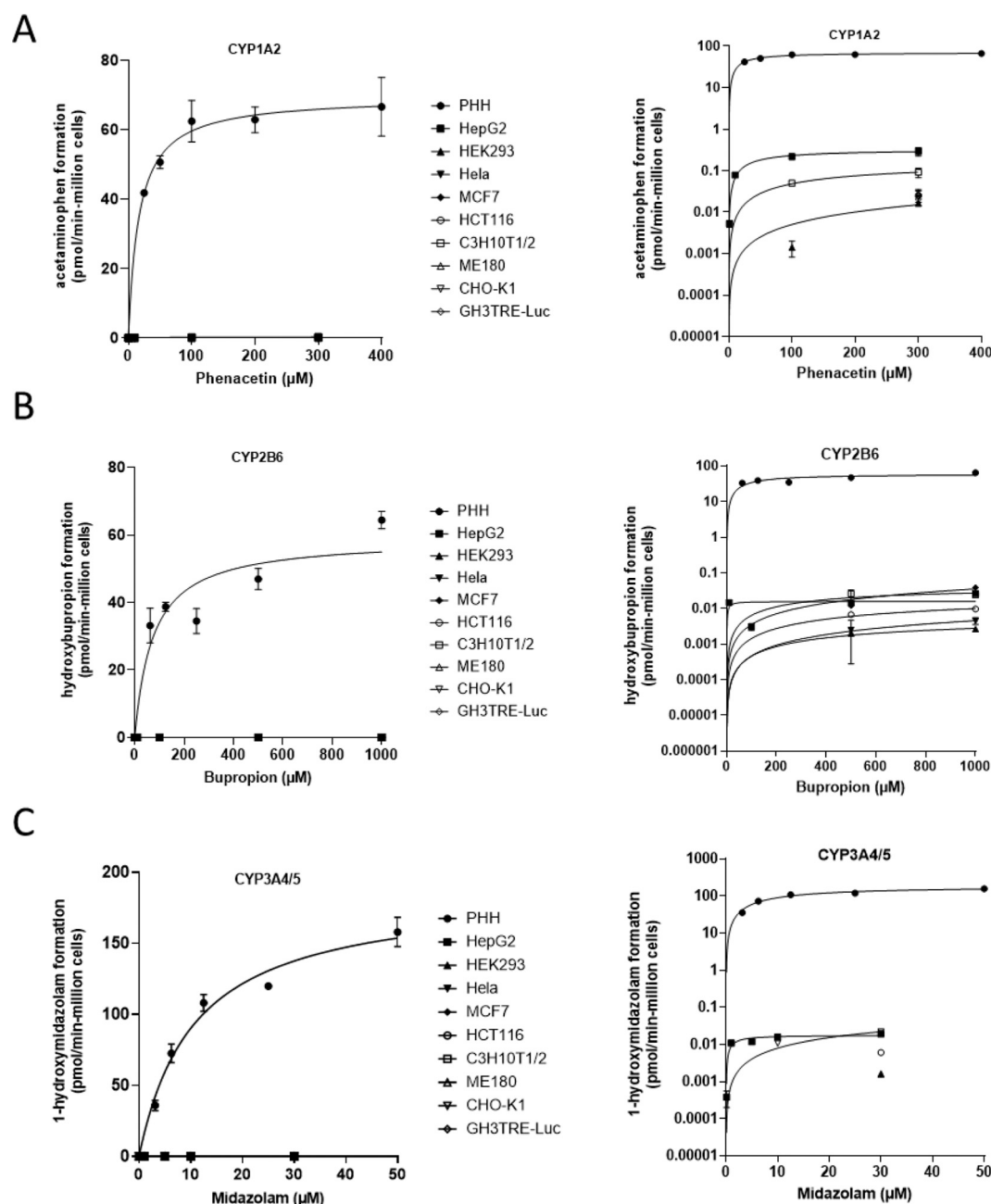
Fig. 1. Metabolism comparison between PHHs and Tox21 cell lines.
