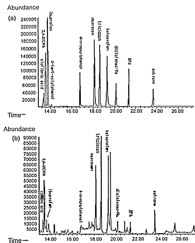
Fig. 2. GC/MSD/SIM chromatograms of extracts from spiked sandy soils (100 ng/g) sample. (a) Extracts with SPE cleanup; (b) without SPE cleanup procedure.
