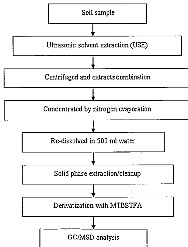
Fig. 1. Scheme of the analytical procedure used for analyzing the target compounds in soil samples.
