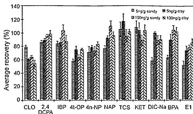
Fig. 3. Percent recovery of target compounds from spiked soil samples extracted with combination of acetone and ethyl acetate ( n=3 ).
