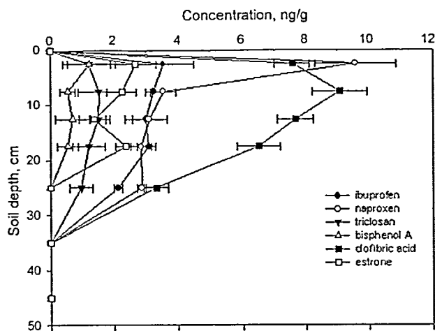
Fig. 4. Vertical concentration profiles of examined compounds in sandy loam soil in a golf course irrigated with reclaimed wastewater.
